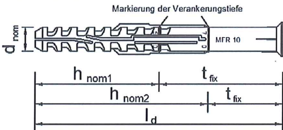
MFR 10 SB
