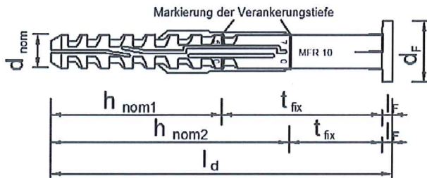
MFR 10 FB
